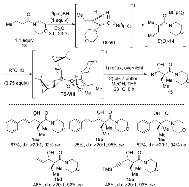
Scheme 4. 1 Reductive aldol reactions of 13 . Reactions were performed with 0.25 mmol of (^d \text{ or } ^l)\text{Ipc}_2\text{BH} at a concentration of 0.25 M. Aldol diastereomer ratios were determined by ^1\text{H} NMR analysis of crude reaction mixture. Only 15 was usually observed. Yields of isolated products are reported. Enantiomeric purity and absolute configuration of the C(3)-hydroxy group was determined by Mosher ester analysis. [16] TMS = trimethylsilyl.
