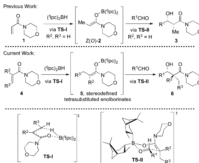
Scheme 1. 1,4-Reductive aldol reactions of substituted \alpha,\beta -unsaturated amides with (Ipc) 2 BH.
