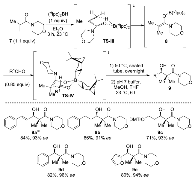
Scheme 2. Reductive aldol reactions of 7 . Reactions were performed with 0.25 mmol of ( d Ipc) 2 BH at a concentration of 0.25 m. Yields of isolated products are reported. Enantiomeric purity and absolute configuration of the C(3)-hydroxy group was determined by Mosher ester analysis. [16] [a] Reaction of 8 with cinnamaldehyde in Et 2 O at reflux using a standard cooling system yielded 9a in similar efficiency (83 %, 92 % ee , performed on 1 mmol scale). DMTr = dimethoxytrityl, THF = tetrahydrofuran.
