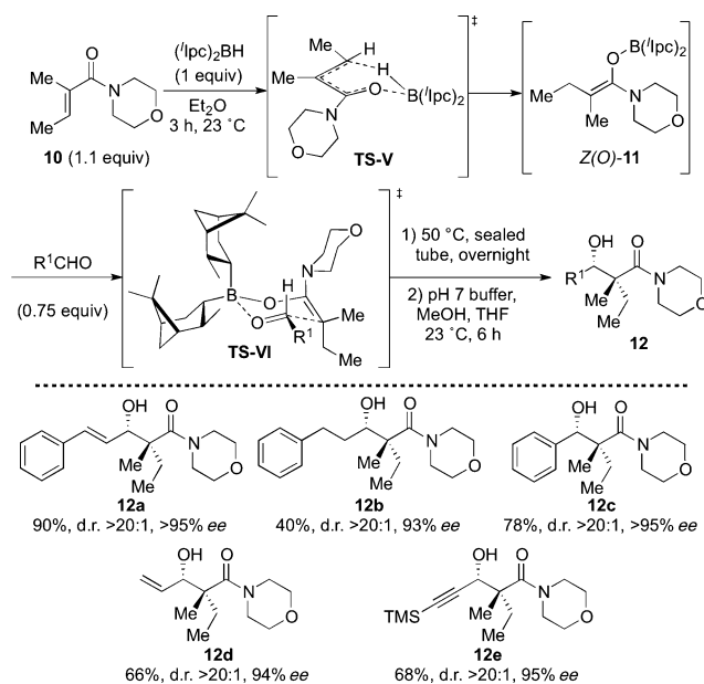
Scheme 3. Reductive aldol reactions of 10 . Reactions were performed with 0.25 mmol of ( l Ipc) 2 BH at a concentration of 0.25 m. Aldol diastereomer ratios were determined by 1 H NMR analysis of crude reaction mixtures. Only 12 was usually observed. Yields of the isolated products are reported. Enantiomeric purity and absolute configuration of the C(3)-hydroxy group was determined by Mosher ester analysis. [16] TMS = trimethylsilyl.
